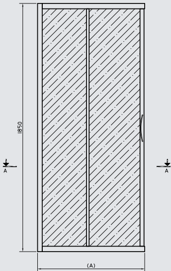
FRONT ELEVATION
